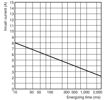
G3R-OD201SN
